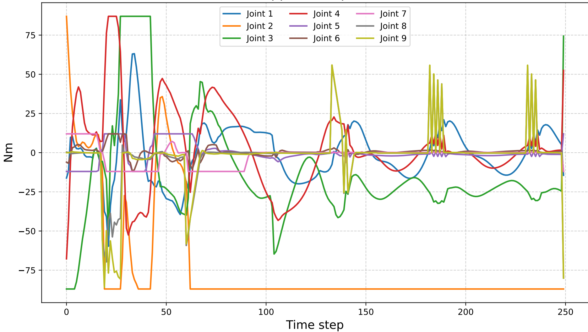
Applied Torques
